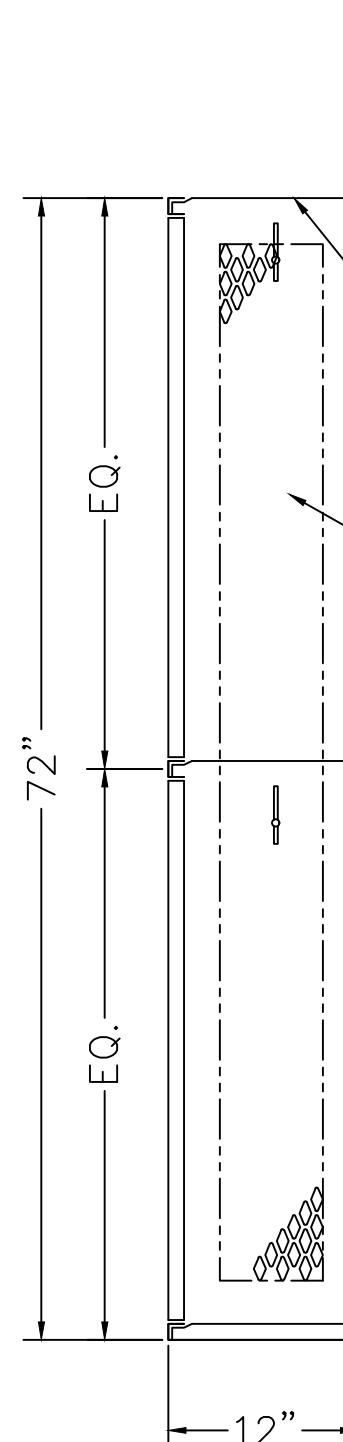
72" EQ. EQ. 12" LOCKER SECTION
