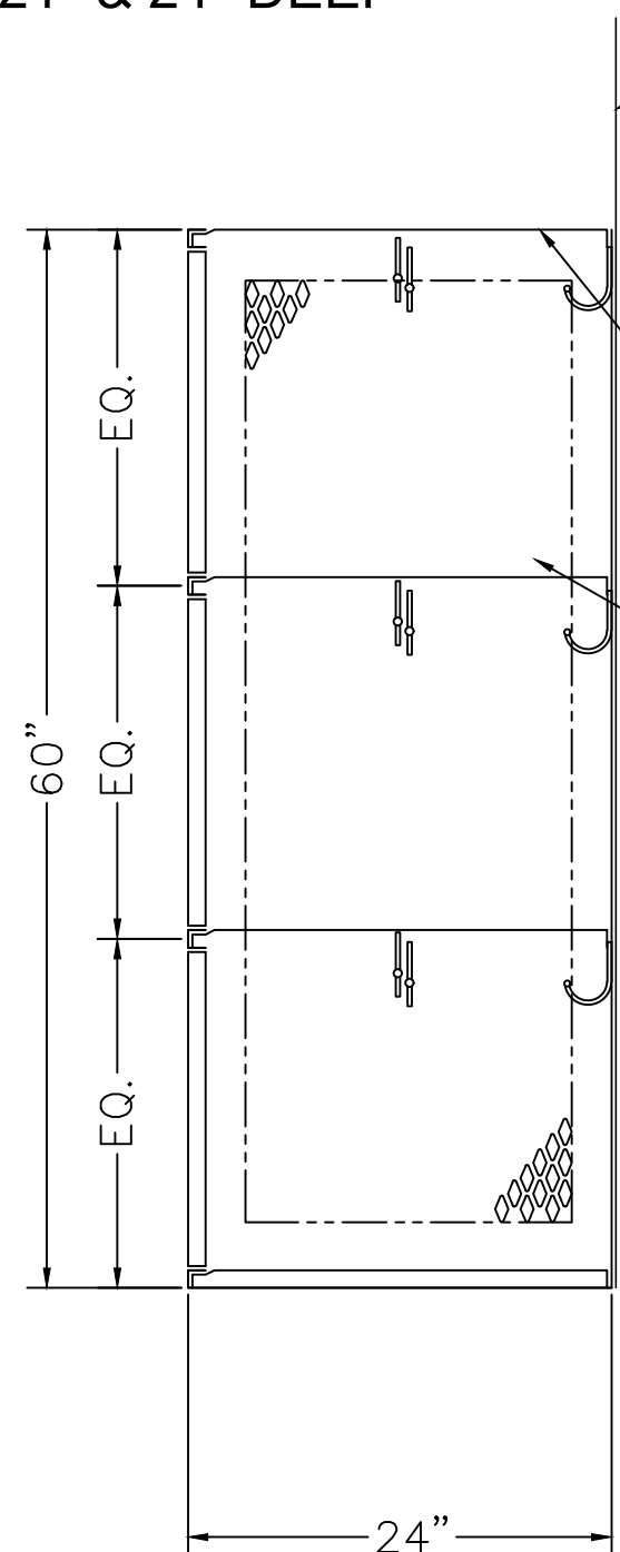
LOCKER SECTION
