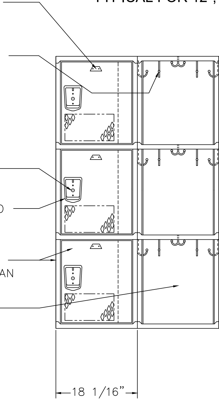
LOCKER ELEVATION
