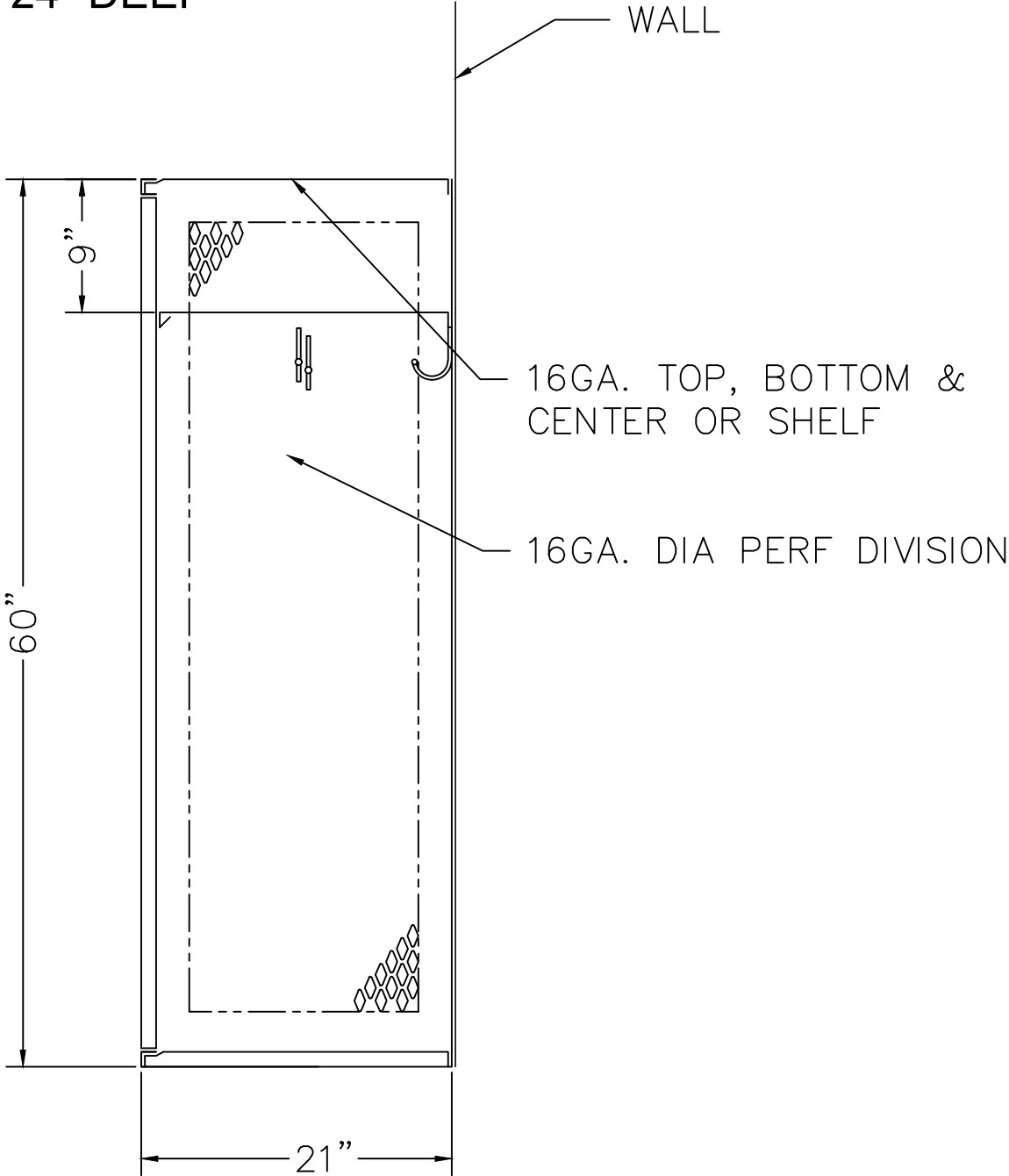
LOCKER SECTION
