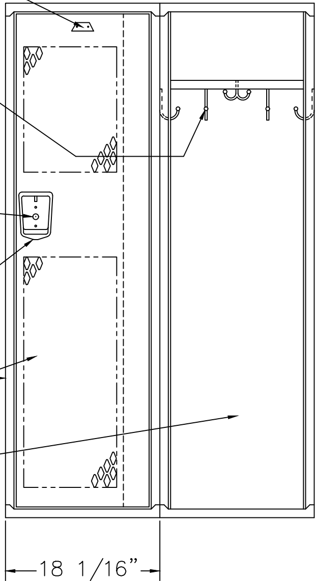
LOCKER ELEVATION
