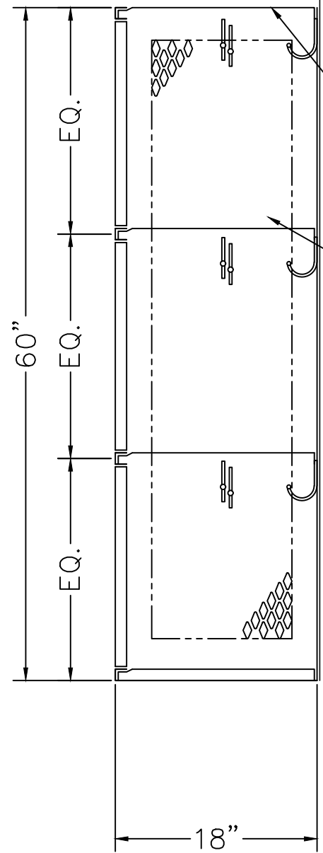
LOCKER SECTION
