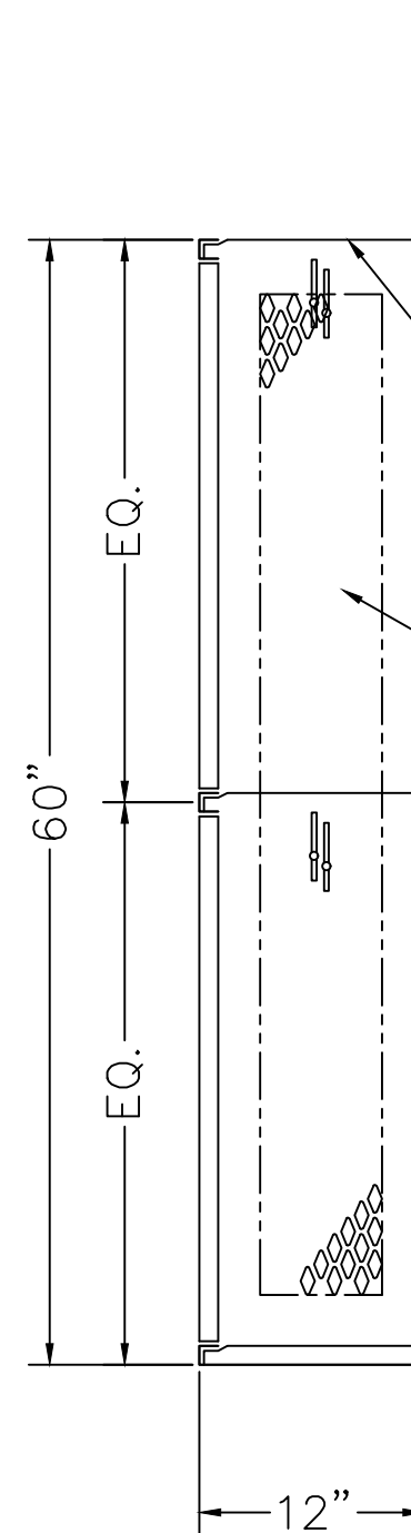
LOCKER SECTION
