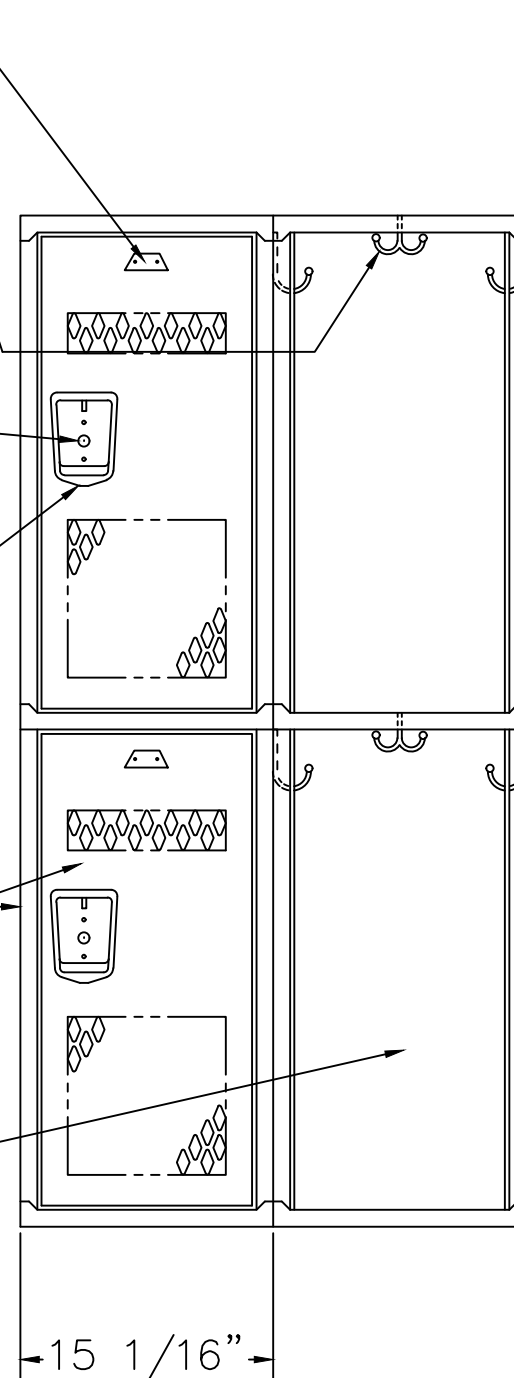
LOCKER ELEVATION
